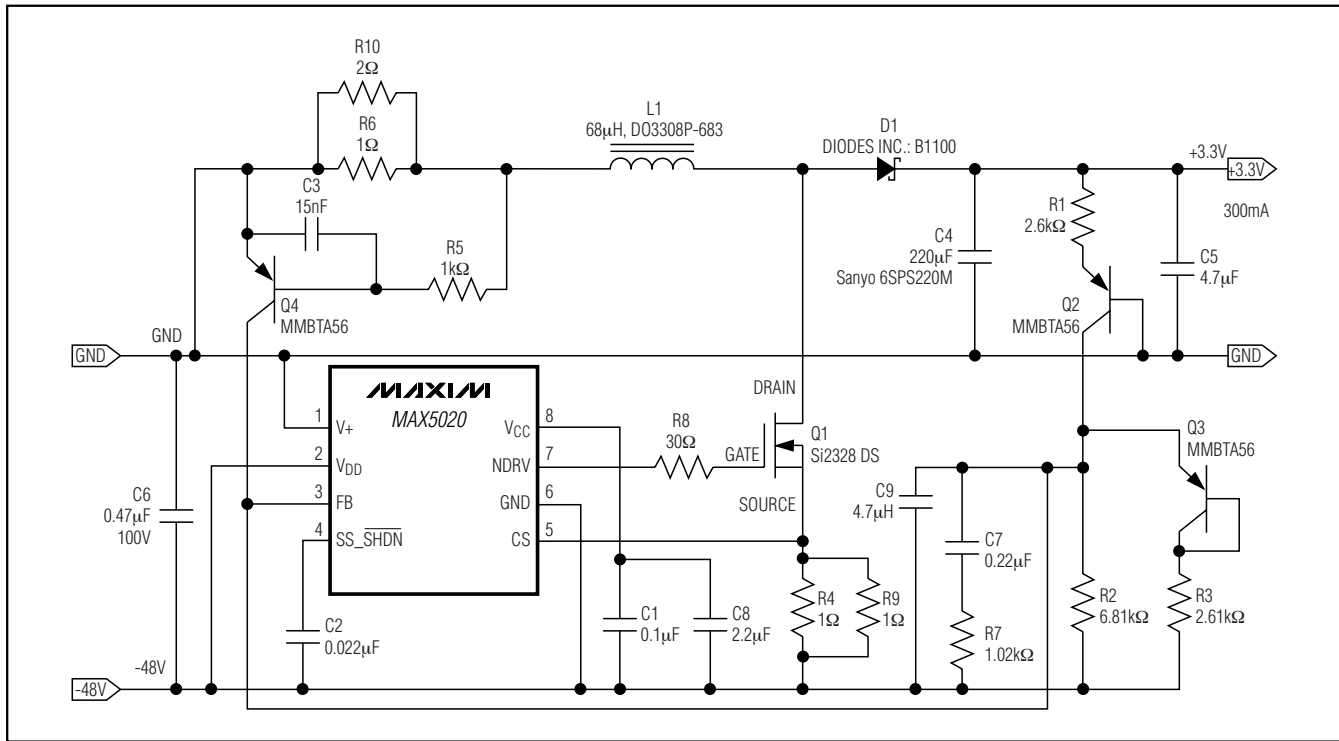
Figure 17. -48V to +3.3V (300mA) Boost Converter Solution for VDI6
