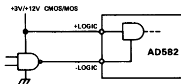
Figure 3B. Inverted Logic Sense Connection
