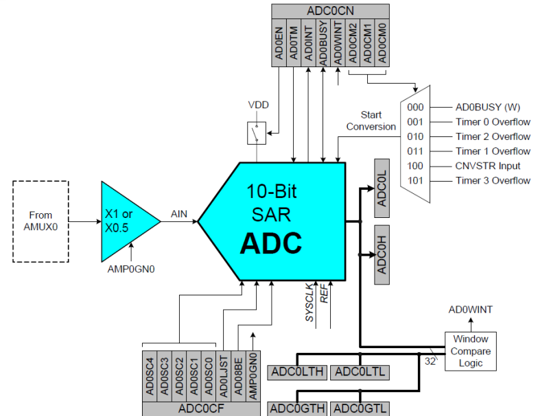
ADC Diagram
