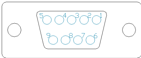
Figure 10: Serial DB9 Connector
