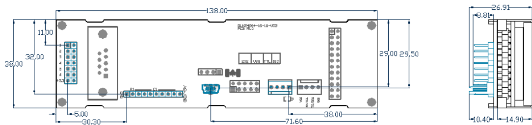
Figure 18: USB Model Dimensional Drawing
