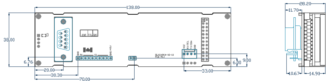
Figure 17: Standard Model Dimensional Drawing
