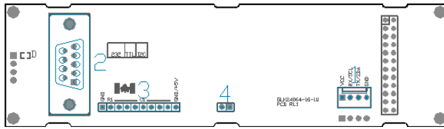
Figure 2: Standard Connections
