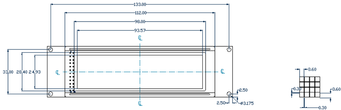
Figure 16: Display Dimensional Drawing
