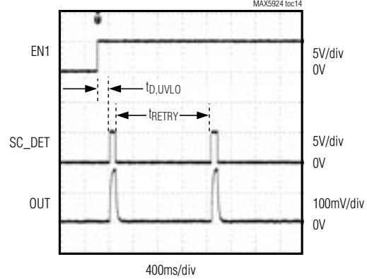
AUTORETRY DELAY
