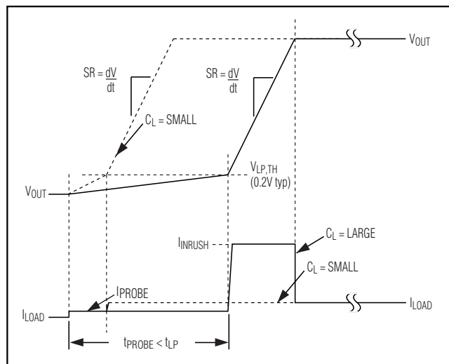
Figure 5. Startup Waveform
