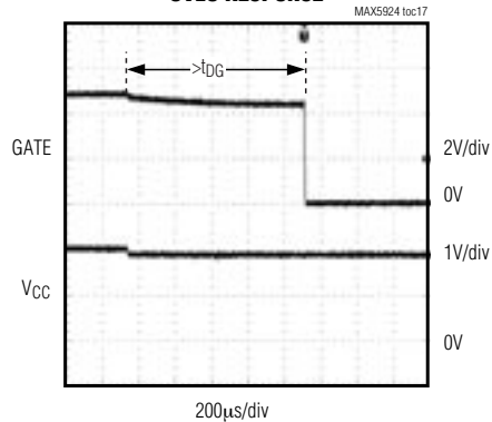
UVLO RESPONSE
