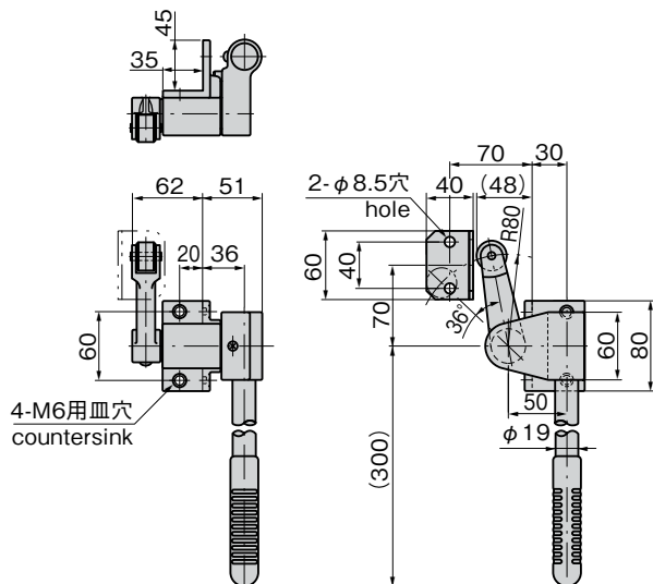
〔FD-150-H-A-R 庫外用〕 Outdoor use
