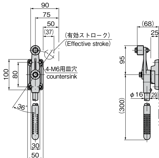
〔FD-150-H-B-R 庫内用〕 Indoor use
