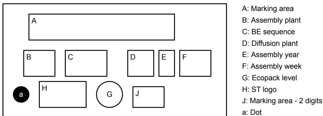
Figure 14. TSSOP28 device package marking area
