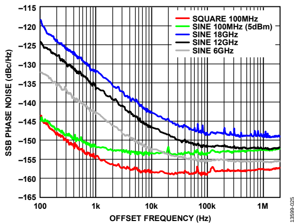
Figure 11. SSB Phase Noise vs. Offset Frequency for Various Input Frequencies, P_{IN} = 0 dBm, T_A = 25^\circ\text{C}
