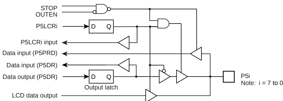
Figure 5-5 Port 5
