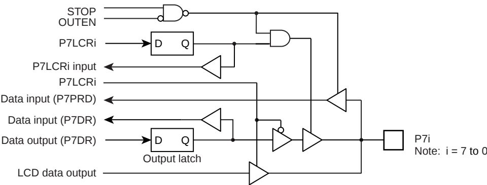
Figure 5-7 Port 7
