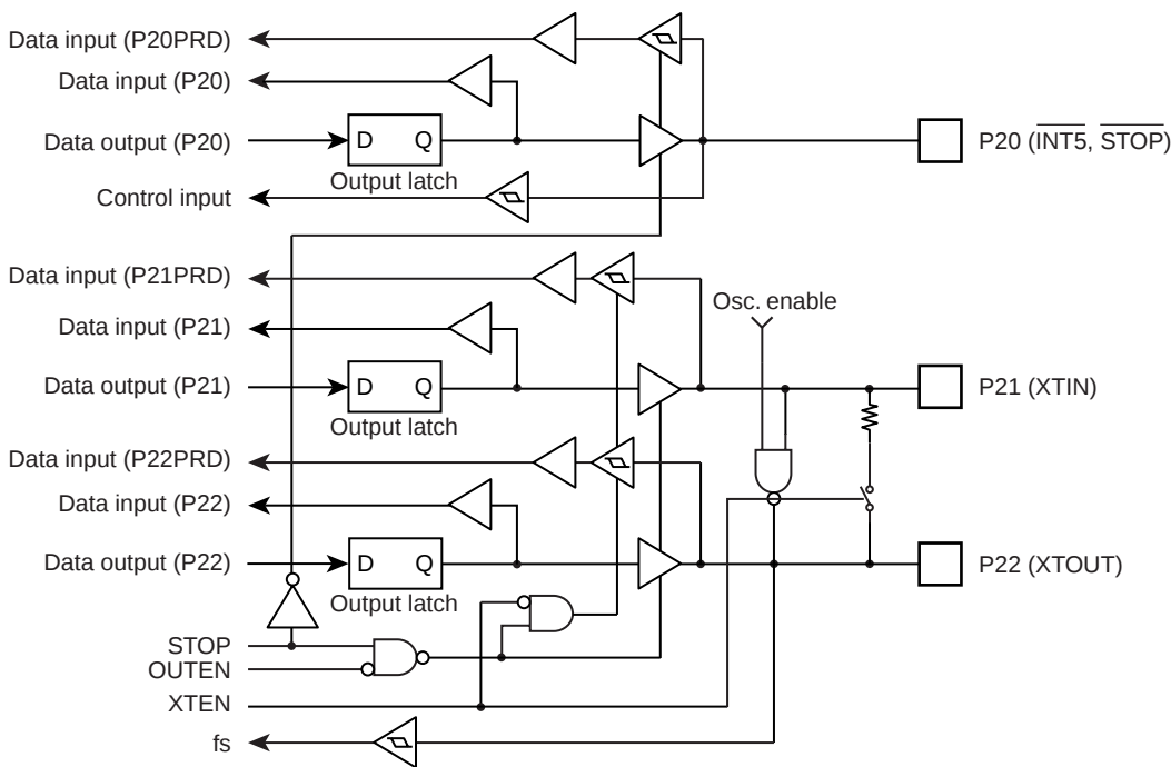
Figure 5-3 Port 2
