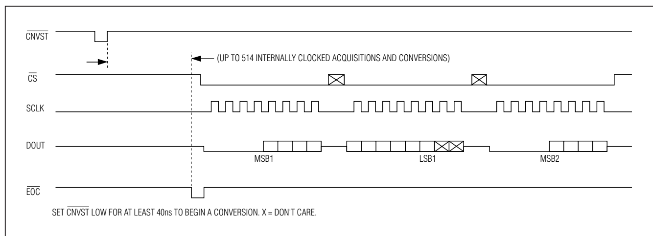
Figure 4. Clock Mode 00
