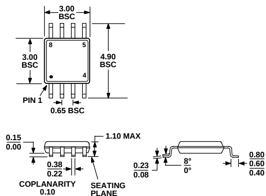
Figure 65. 8-Lead Standard Small Outline Package [MSOP] (RM-8) Dimensions shown in millimeters
