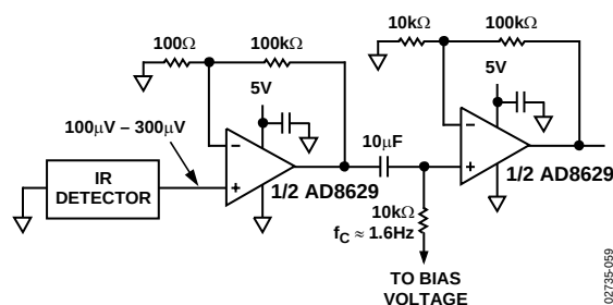
Figure 62. AD8629 Used as Preamplifier for Thermopile
