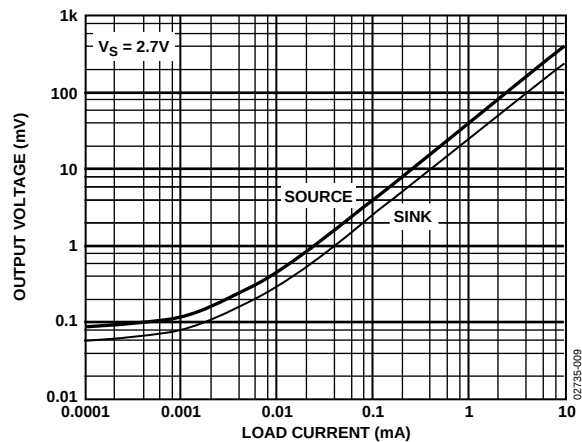
Figure 11. Output Voltage to Supply Rail vs. Load Current at 2.7 V
