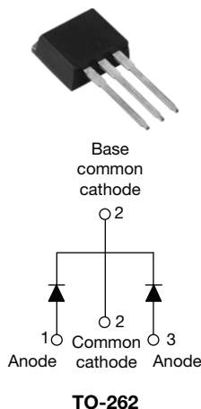
VS-25CTQ...-1PbF
