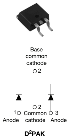
VS-25CTQ...SPbF
