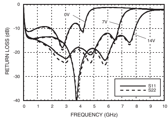
Return Loss vs. Control Voltage [1]
