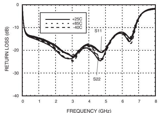
Return Loss vs. Temperature, Vctl @ 7V [1]
