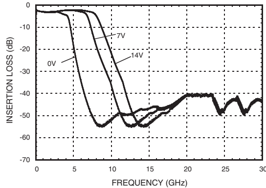
Broadband Insertion Loss vs. Control Voltage
