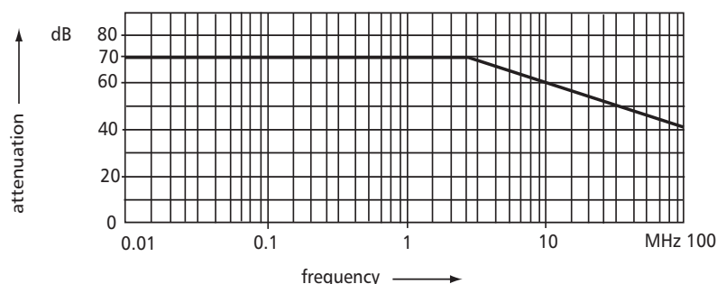
Shielding Characteristics
