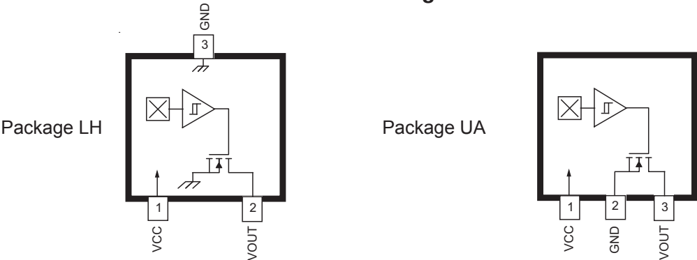
Terminal List
