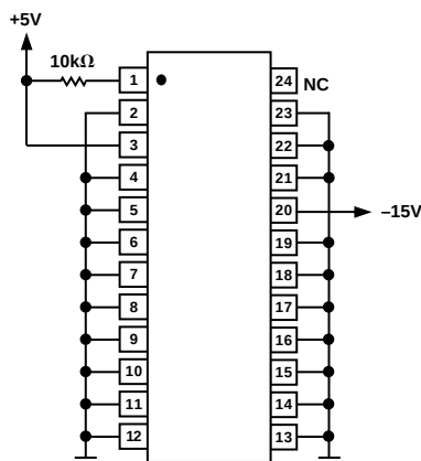
Figure 2. Burn-In Diagram
