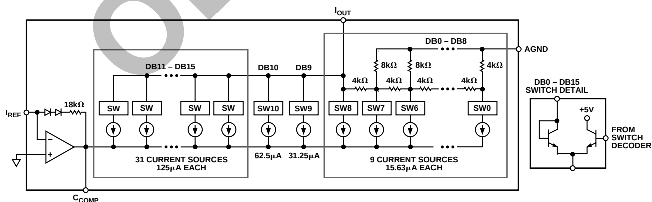
Figure 3. DAC16 Architecture
