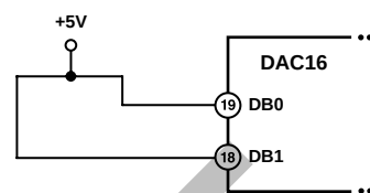
Figure 6. Handling Unused DAC16 Digital Inputs
