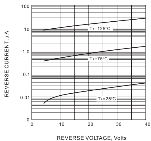
FIG. 2-TYPICAL REVERSE CHARACTERISTICS
