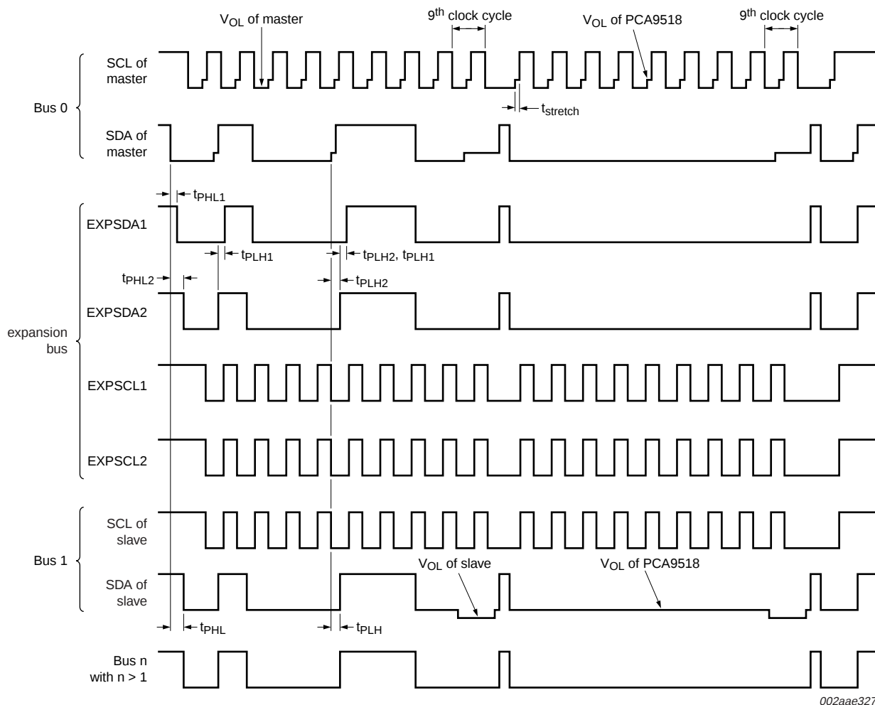
Fig 6. Bus waveforms
