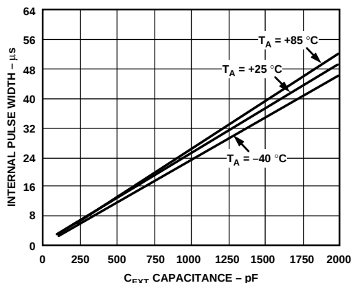
Figure 7. Internal Pulse Width vs. \text{C}_{\text{EXT}}
