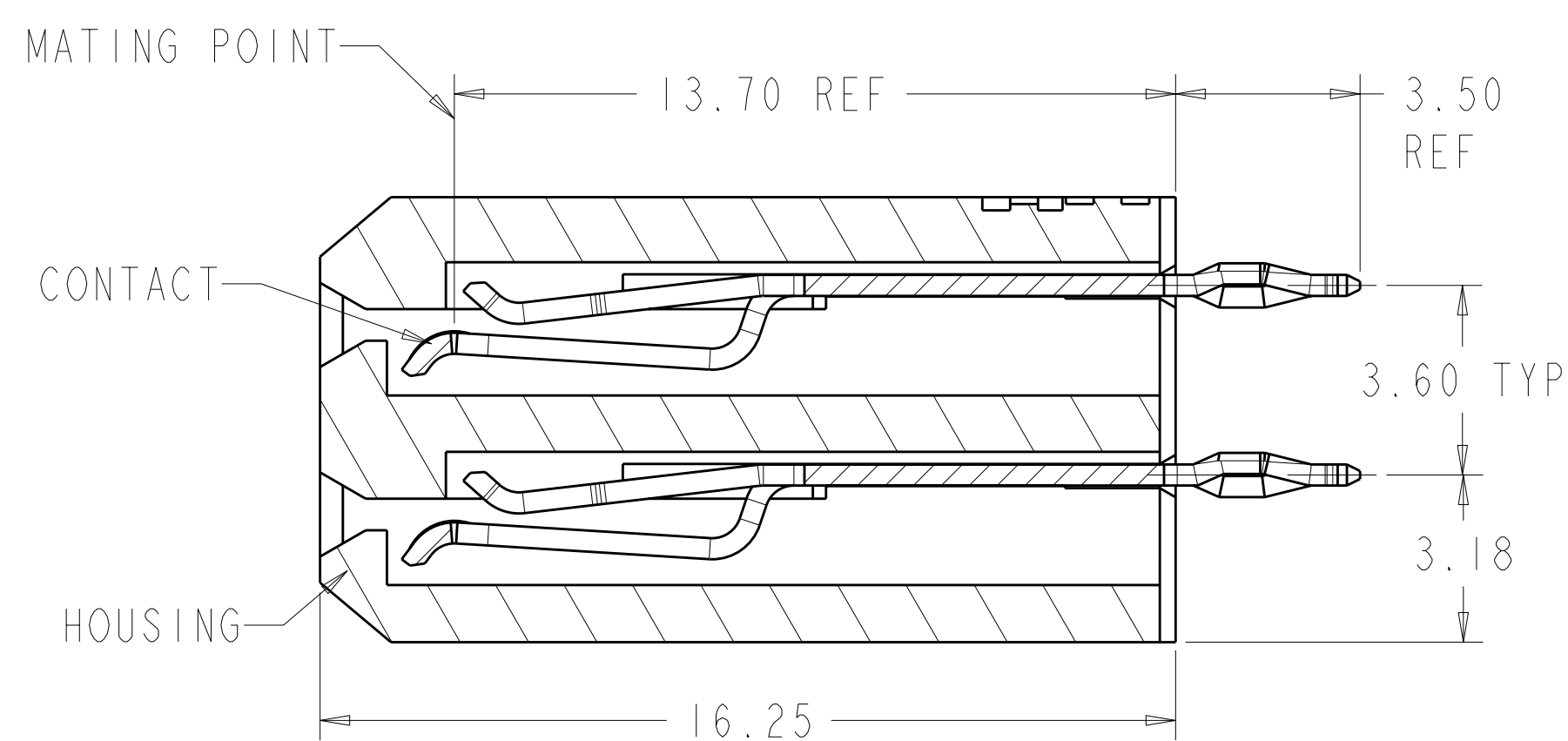
PIN "1a"
