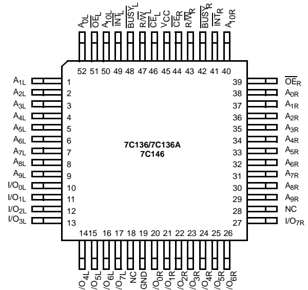
Figure 2. 52-Pin PQFP (Top View)
