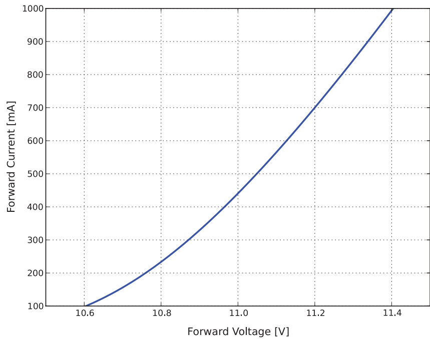
Figure 11. Forward current vs. forward voltage.
