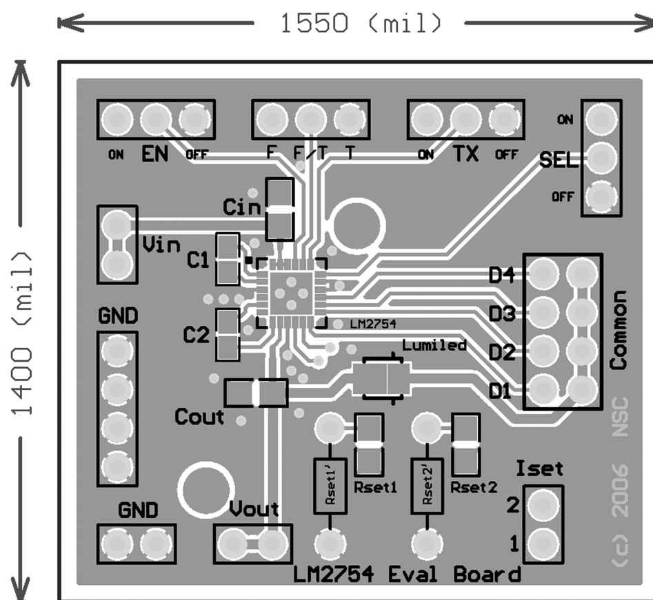
Figure 1. Top Layer
