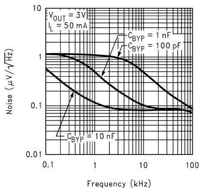
Figure 5-45. Output Noise Density (Legacy Chip)
