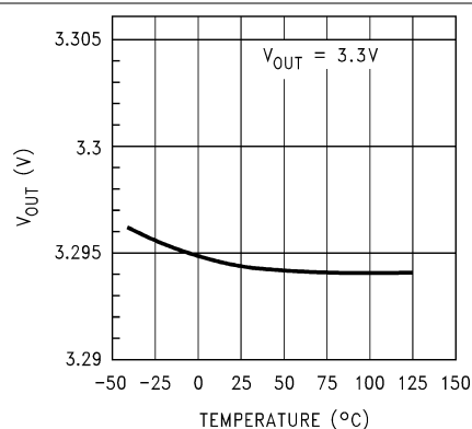
Figure 5-2. Output Voltage vs Temperature (Legacy Chip)
