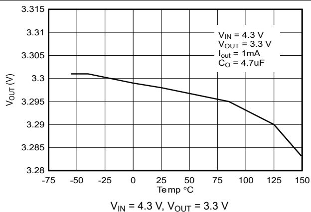
Figure 5-4. Output Voltage vs Temperature (New Chip)
