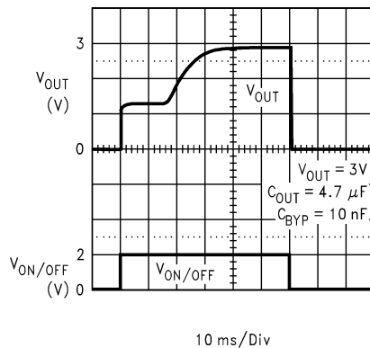
Figure 7-17. Turnon Waveform (Legacy chip)
