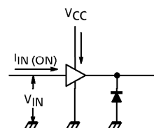
3. I_{IN(ON)} , I_{CC}
