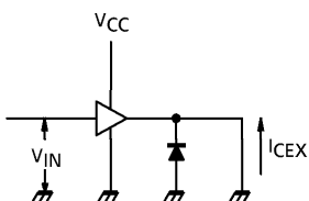
4. V_{IN(ON)} , V_{IN(OFF)}
