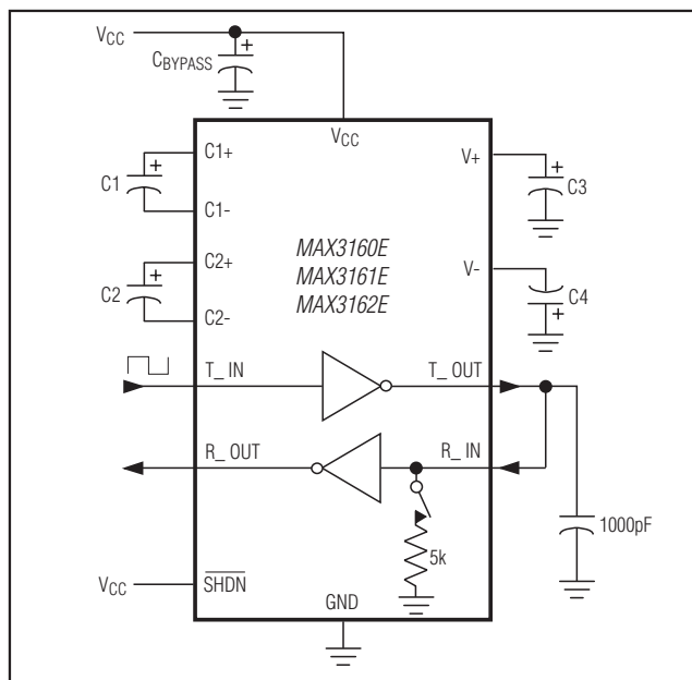
Figure 14. Loopback Test Circuit
