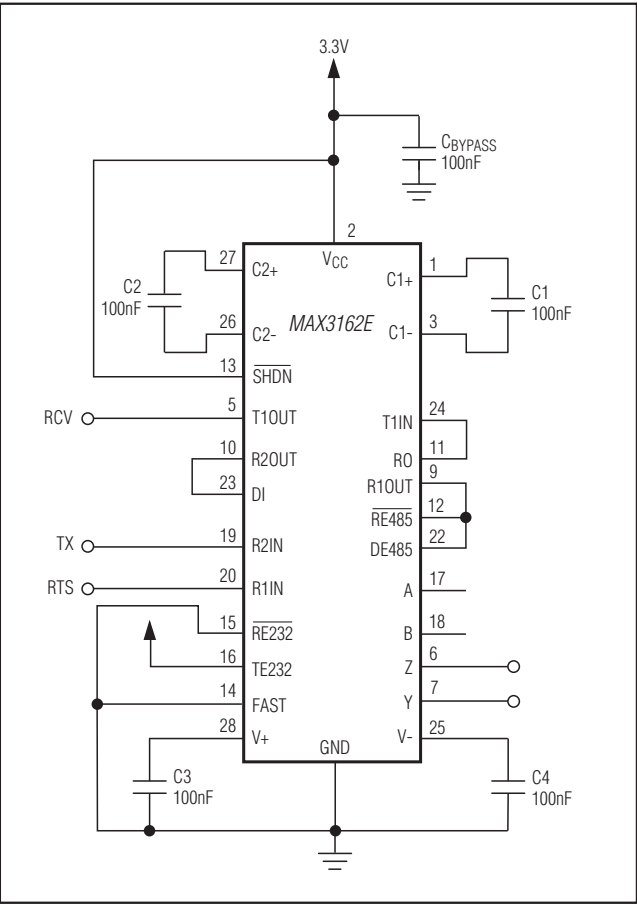
Figure 18. Protocol Translator
