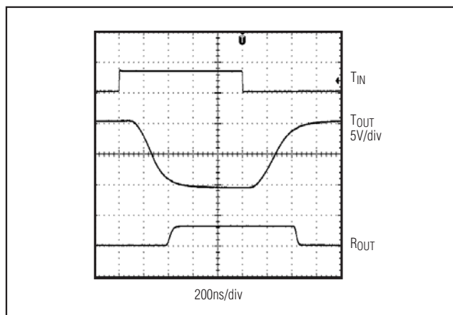
Figure 16. MAX3161E/MAX3162E RS-232 Loopback Test Result at 1Mbps, FAST = High
