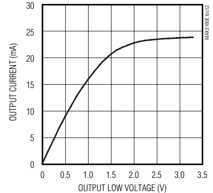
RECEIVER OUTPUT CURRENT vs. RECEIVER- OUTPUT LOW VOLTAGE
