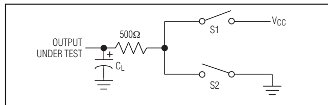
Figure 4. RS-485/RS-422 Driver Enable/Disable Timing Test Load
