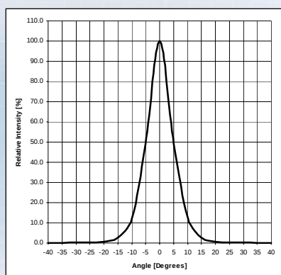
Radiation Pattern with 5° optic (CW)
