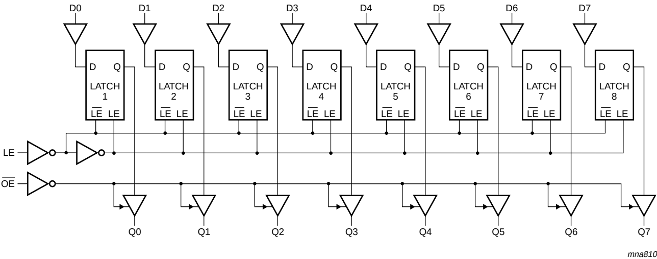
Fig 5. Logic diagram
