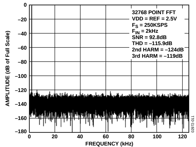
Figure 12. FFT Plot
