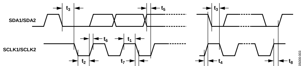
Figure 3. I²C Timing
