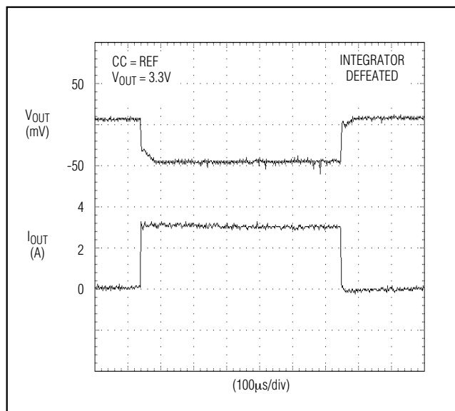
Figure 5b. Load-Transient Response with Integrator Deactivated
