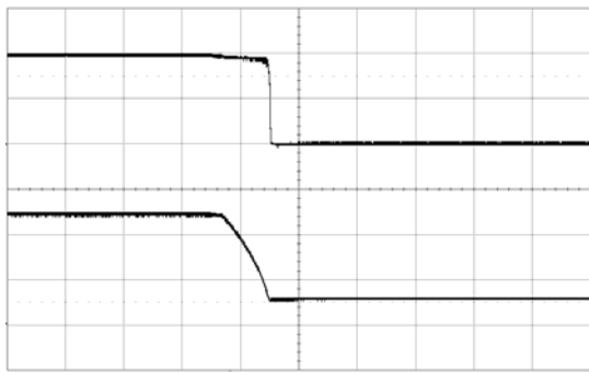
Shut-down enabled by disconnecting V_I at: T_{P1} = +25\text{ }^{\circ}\text{C} , V_I = 12\text{ V} , V_O = 1.0\text{ V} C_O = 470\text{ }\mu\text{F}/10\text{ m}\Omega , I_O = 20\text{ A} Top trace: output voltage (0.5 V/div.). Bottom trace: input voltage (5 V/div.). Time scale: (2 ms/div.).
