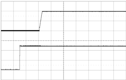
Start-up enabled by connecting V_I at: T_{P1} = +25\text{ }^{\circ}\text{C} , V_I = 12\text{ V} , V_O = 1.0\text{ V} C_O = 470\text{ }\mu\text{F}/10\text{ m}\Omega , I_O = 20\text{ A} Top trace: output voltage (0.5 V/div.). Bottom trace: input voltage (5 V/div.). Time scale: (20 ms/div.).
