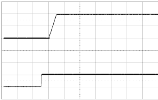
Start-up by enabling CTRL signal at: T_{P1} = +25\text{ }^{\circ}\text{C} , V_I = 12\text{ V} , V_O = 1.0\text{ V} C_O = 470\text{ }\mu\text{F}/10\text{ m}\Omega , I_O = 20\text{ A} Top trace: output voltage (0.5 V/div.). Bottom trace: CTRL signal (5 V/div.). Time scale: (20 ms/div.).
