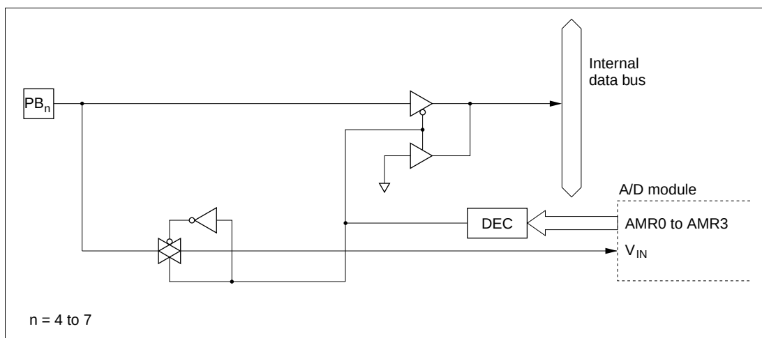
Figure C.9 Port B Block Diagram
