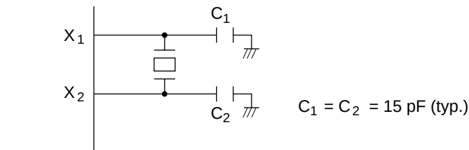
Figure 4.7 Typical Connection to 32.768-kHz Crystal Oscillator
