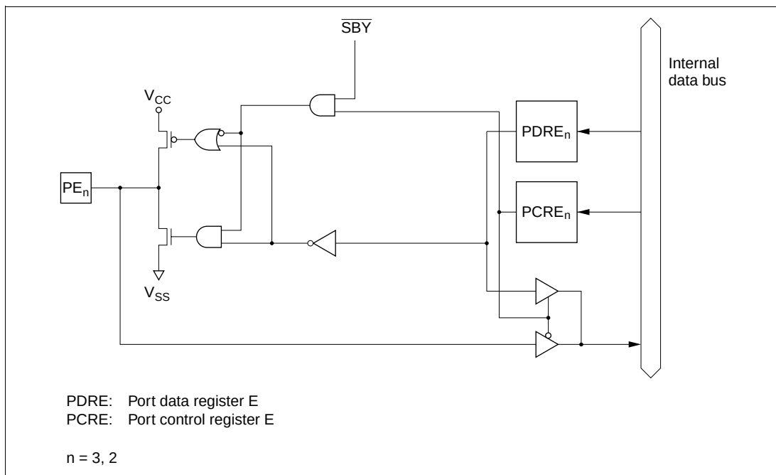
Figure C.10 Port E Block Diagram
