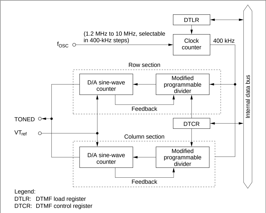
Figure 11.2 DTMF Generator Block Diagram
