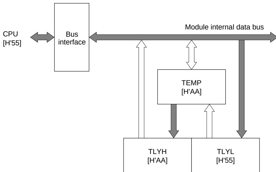
Figure 9.16 TLY Write Operation (CPU → TLY)
