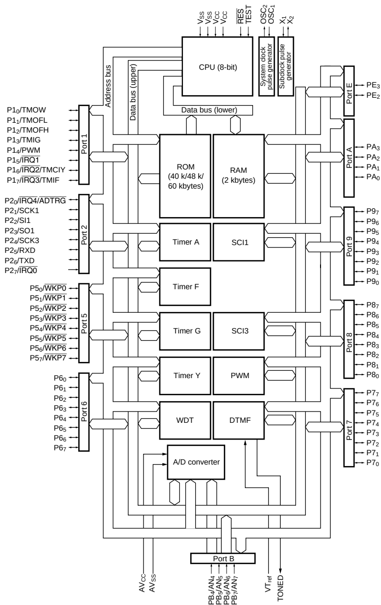
Figure 1.1 Block Diagram
