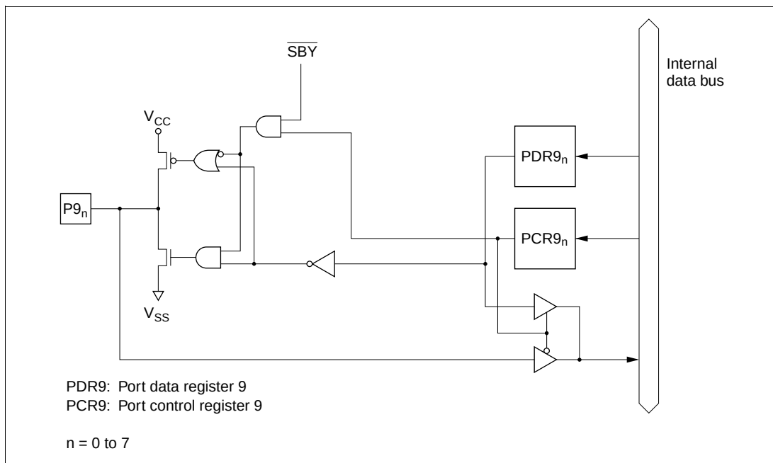
Figure C.7 Port 9 Block Diagram
