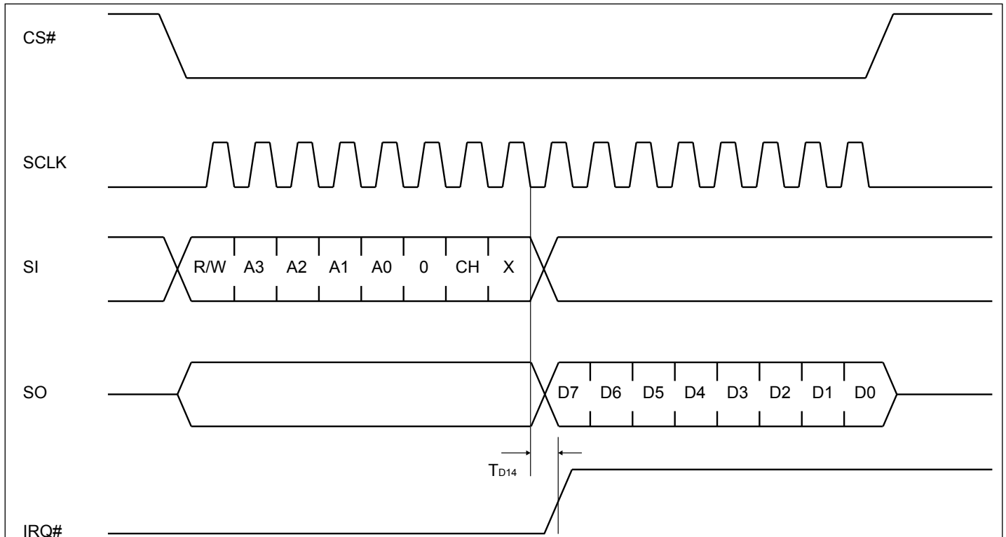
Figure 15. Read RHR To Clear RX INT
