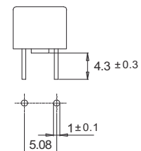
Dimensions [mm]
