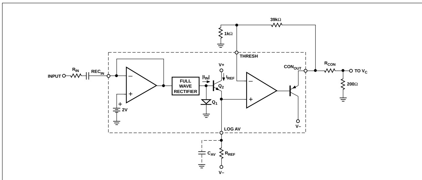
FIGURE 2: Level Detector
