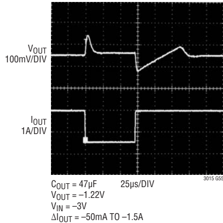
LT3015 Transient Response, C_{OUT} = 47\mu\text{F}
