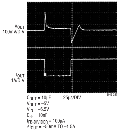
LT3015 Transient Response, C_{FF} = 10\text{nF} , C_{OUT} = 10\mu\text{F}
