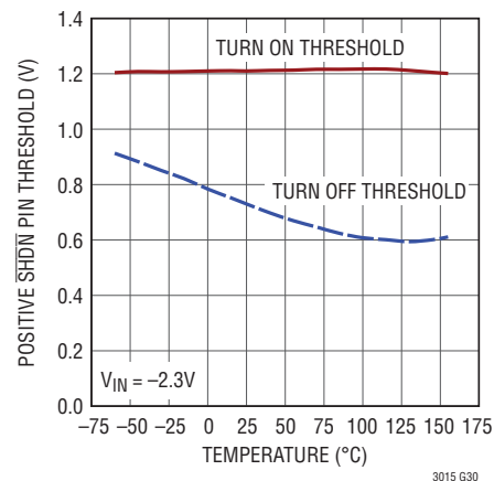
Positive \overline{\text{SHDN}} Pin Thresholds
