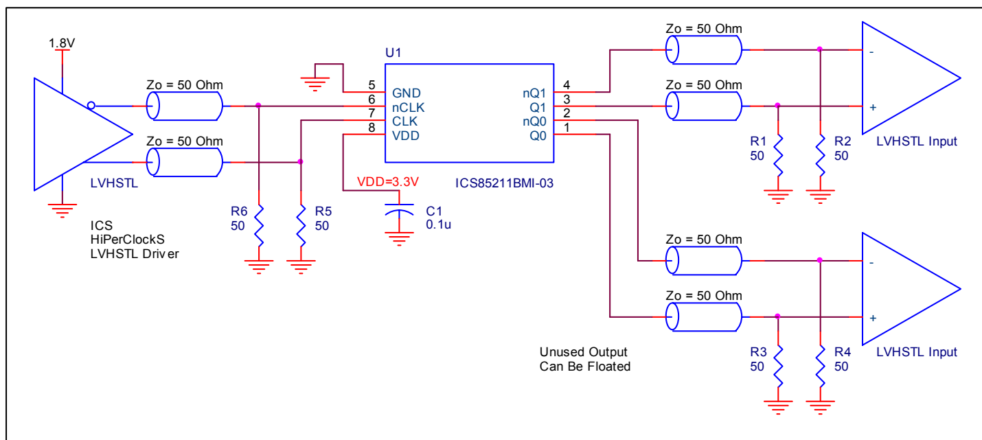
Figure 3. ICS85211BI-03 LVHSTL Buffer Schematic Example
