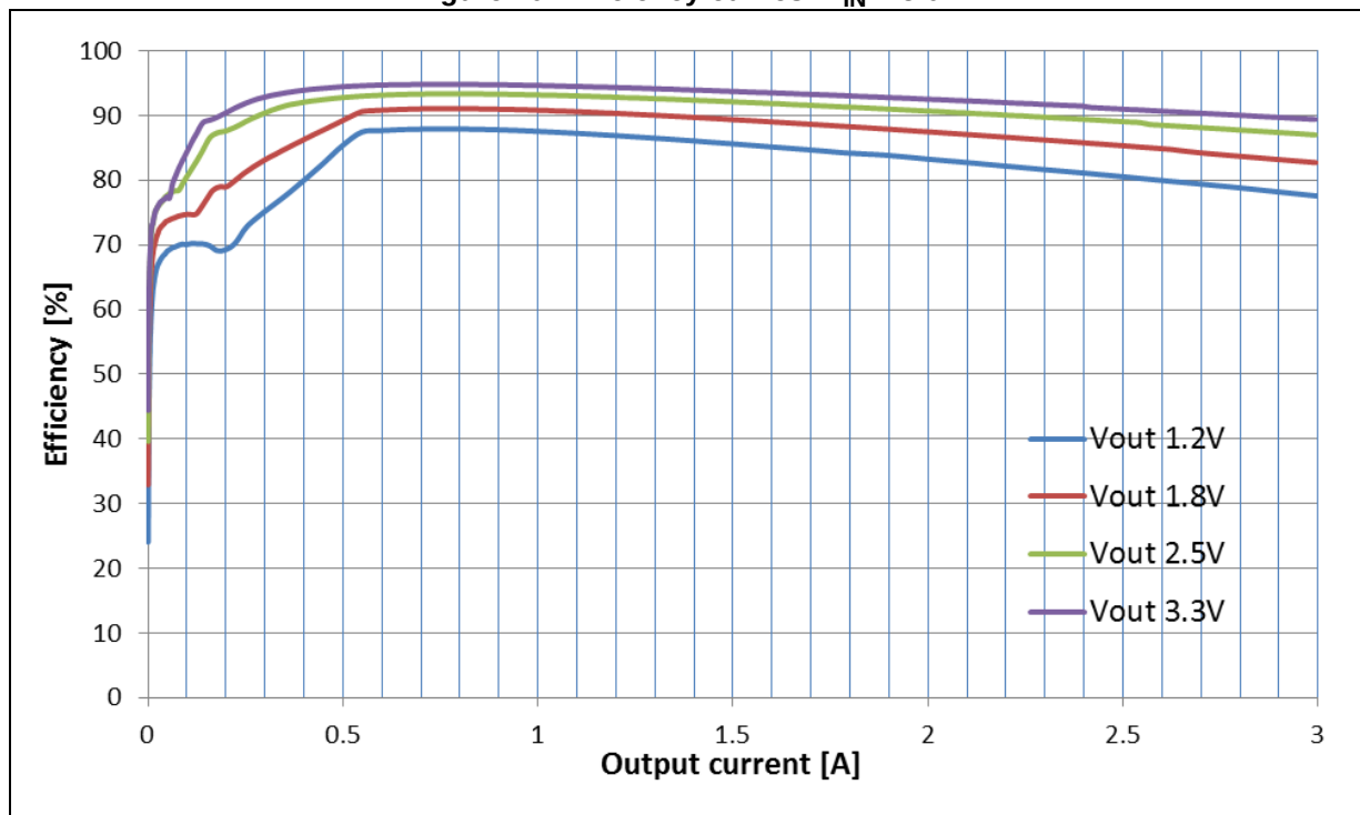
Figure 20. Efficiency curves: V_{IN} = 5.0\text{ V}
