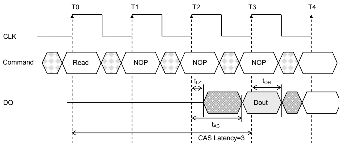
Figure 2. CAS Latency
