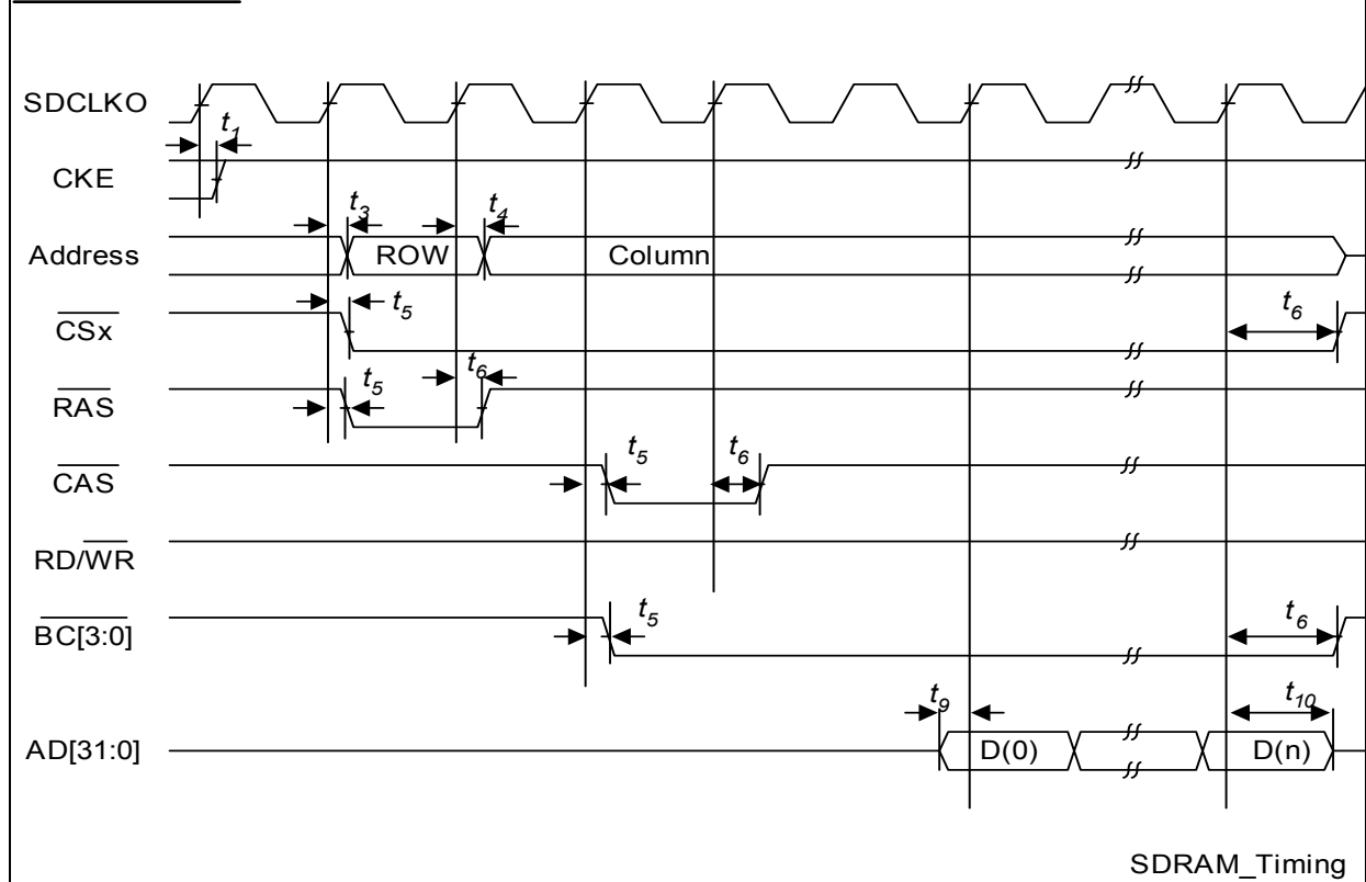
Figure 4-10 SDRAM Access Timing
