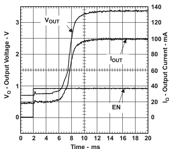
TPS61006 Start-Up Timing Into 33- \Omega Load
