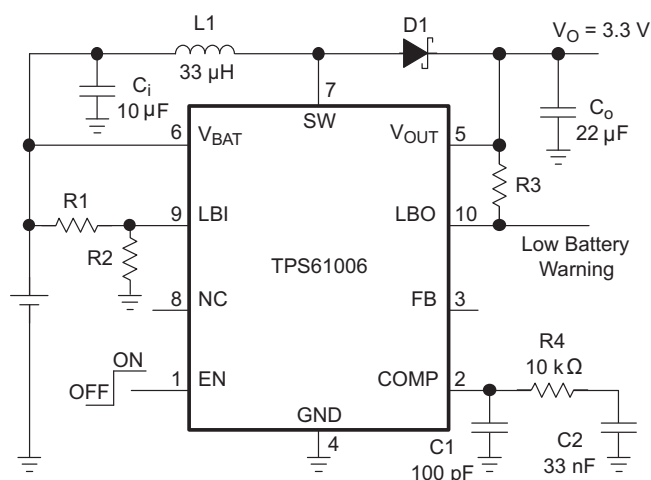
Typical Application Circuit for Fixed Output Voltage Options
