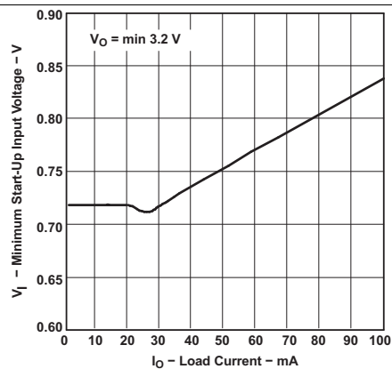
Figure 10. Minimum Start-up Input Voltage vs Load Current
