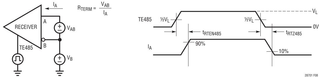
Figure 8. RS485 Termination Resistance and Timing Measurements (Note 5)
