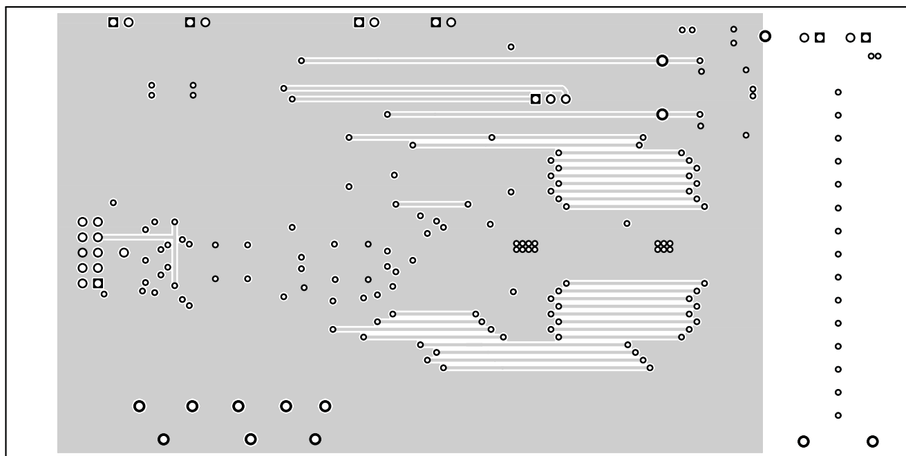
Figure 4. Layer 2 Routing
