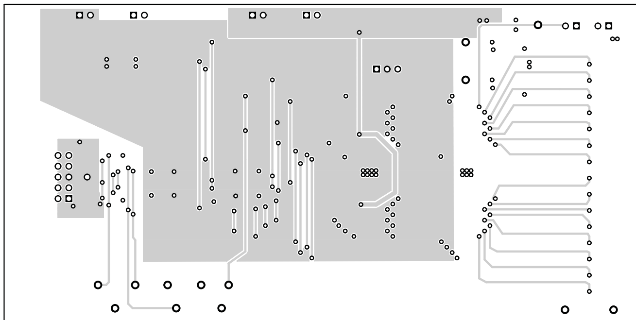
Figure 5. Layer 3 Routing
