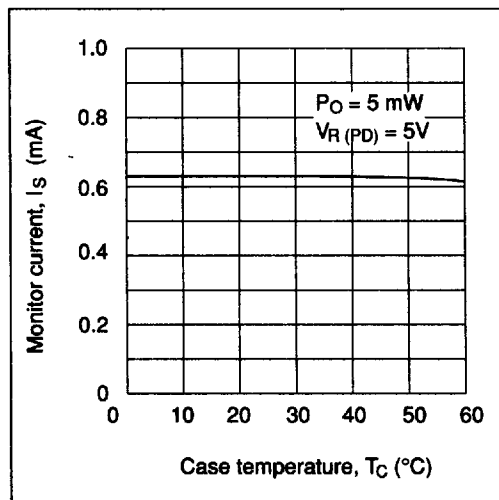
Figure 9 Monitor Current vs. Case Temperature (HL7832HG)
