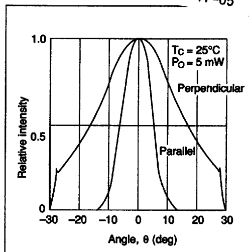
Figure 4 Far Field Pattern (HL7832HG)
