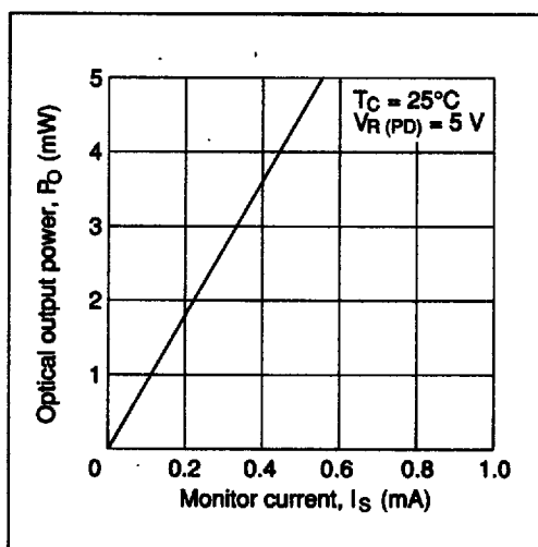
Figure 6 Optical Output Power vs. Monitor Current (HL7832HG)
