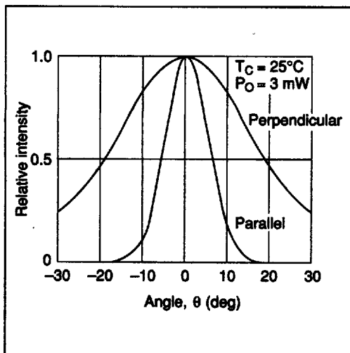
Figure 3 Far Field Pattern (HL7832G)
