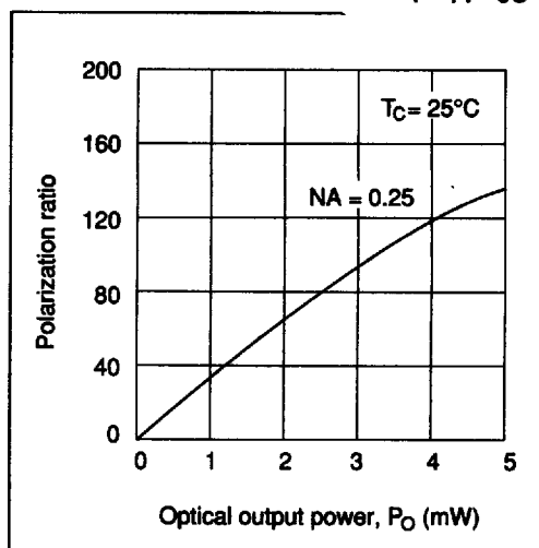
Figure 12 Polarization Ratio vs. Optical Output Power (HL7832HG)
