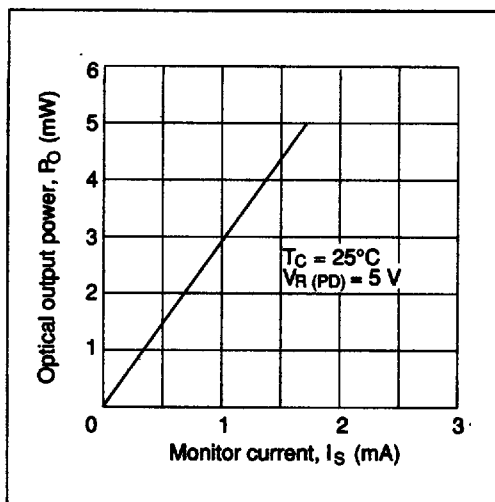
Figure 5 Optical Output Power vs. Monitor Current (HL7832G)
