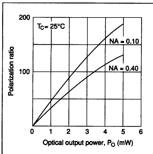
Figure 11 Polarization Ratio vs. Optical Output Power (HL7832G)
