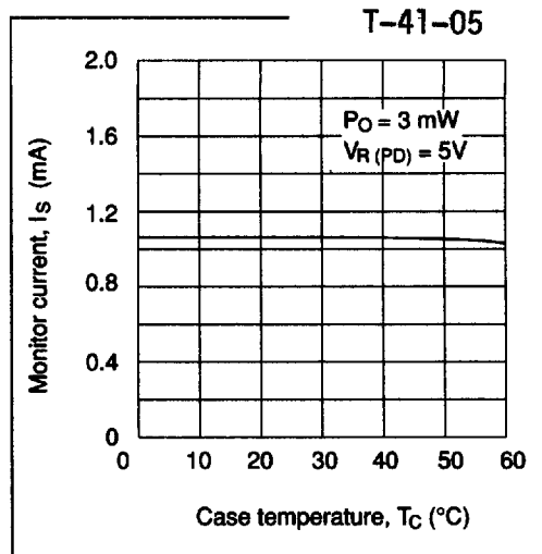
Figure 8 Monitor Current vs. Case Temperature (HL7832G)
