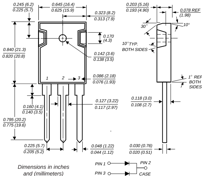
TO-247AD (TO-3P)
