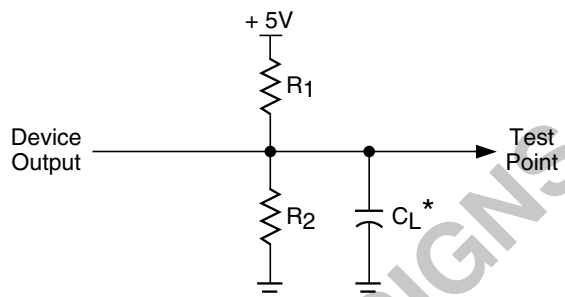
Figure 2. Test Load
