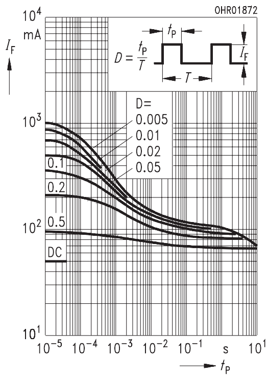
Figure 5. Permissible Pulse Handling Capability, I_F = f(t_P) , duty cycle D = \text{parameter} , T_A = 25^\circ\text{C}
