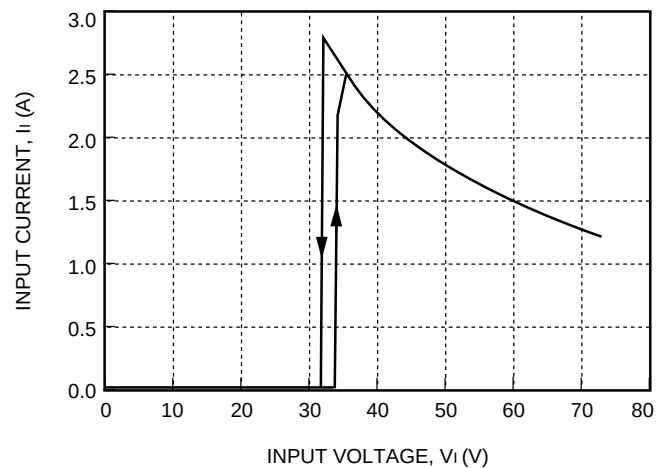
Figure 2. Typical JW075A Input Characteristics at Room Temperature
