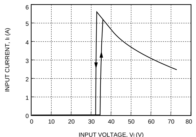
Figure 4. Typical JW150A Input Characteristics at Room Temperature
