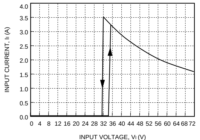
Figure 3. Typical JW100A Input Characteristics at Room Temperature
