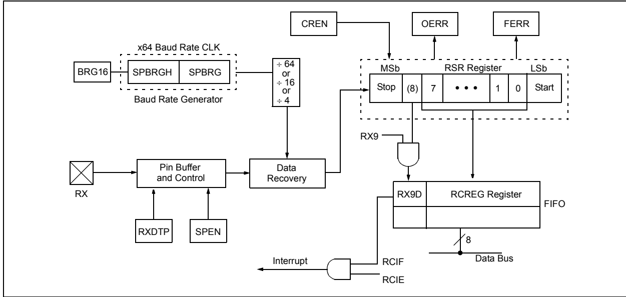
FIGURE 20-7: ASYNCHRONOUS RECEPTION, RXDTP = 0 (RX NOT INVERTED)
